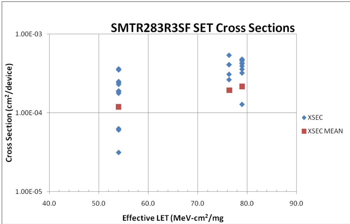
Chart 3. SMTR283R3S SET Cross Sections
