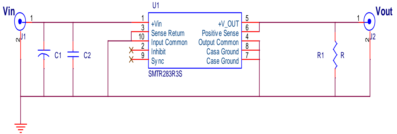
Figure 2. Overall Block Diagram for the testing of the SMTR283R3S
