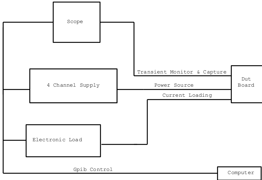
Figure 1. Overall Block Diagram for the testing of the SMTR283R3S
