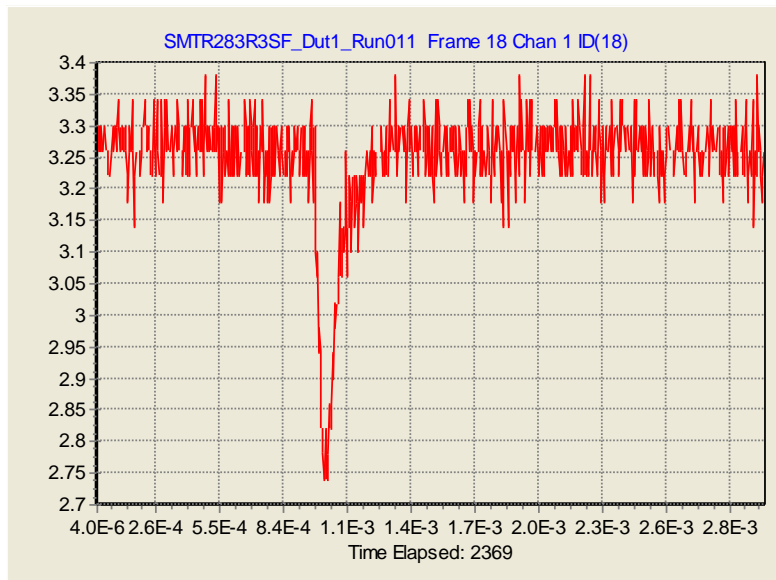
Chart 2. Typical Worst Case Width Transient of < 100us
