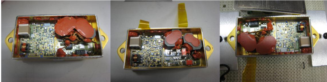
Figure 3. SMTR283R3S internal circuitry exposed for ion beam test at TAMU
